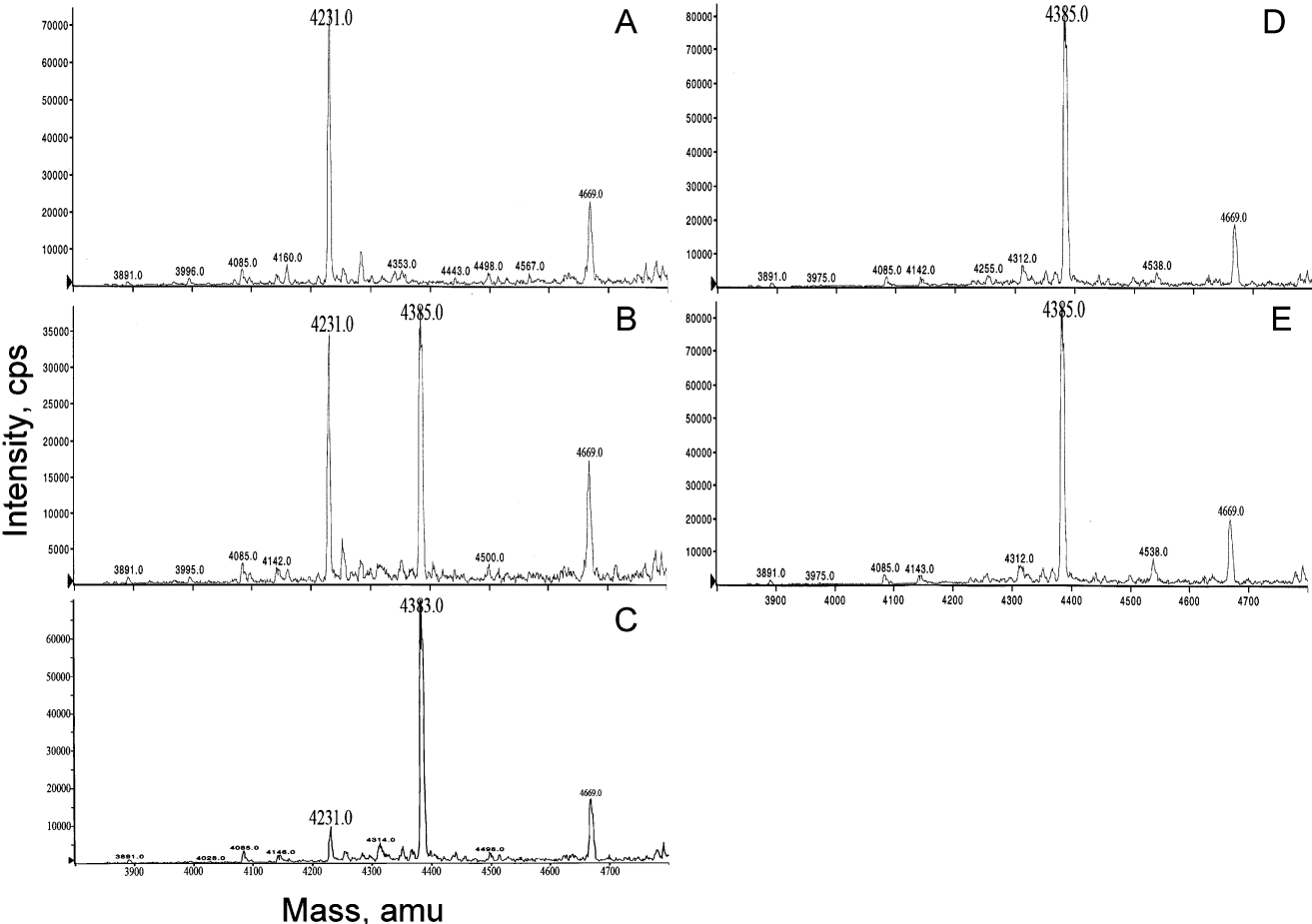
FIGURE 3: Relative quantitation of Gd chelation to DTPA[N-4ab/Q-4ab]Aβ30 by electrospray ionization mass spectrometry. Mixtures of increasing mole ratios of Gd to DTPA[N-4ab/Q-4ab]Aβ30 were analyzed: (A) 0/1, (B) 0.25/1, (C) 0.5/1, (D) 0.75/1, and (E) 1/1. See the text for details.
