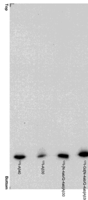
FIGURE 2: Autoradiography after SDS-PAGE of [ ^{125}\text{I} ]A \beta derivatives. SDS-polyacrylamide gel electrophoresis of radioiodinated A \beta peptides and derivatives.
