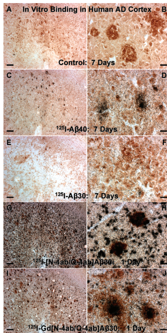
FIGURE 4: Labeling of amyloid plaques in human AD brain sections in vitro . (A and B) Unfixed temporal lobe cortex section incubated with buffer only and processed for anti-A \beta IH and emulsion autoradiography (exposed for 7 days). (C and D) Sections incubated with 100 pM [ 125 I]A \beta 40 (exposed for 7 days). (E and F) Section incubated with 100 pM [ 125 I]A \beta 30 (exposed for 7 days). (G and H) Section incubated with 100 pM [ 125 I][N-4ab/Q-4ab]A \beta 30 (exposed for 1 day). (I and J) Section incubated with 100 pM [ 125 I]Gd[N-4ab/Q-4ab]A \beta 30 (exposed for 1 day). For panels A, C, E, G, and I, the scale bar is 250 \mu m. For panels B, D, F, H, and J, the scale bar is 25 \mu m.
