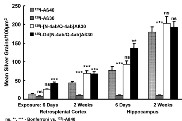
FIGURE 10: Quantitation of exposed silver grains on amyloid plaques in the retrosplenial cortex and hippocampus of 21-month-old APP, PS1 mice. On the ordinate is plotted the mean number of exposed silver grains per 100 \mu\text{m}^2 quantitated by stereological methods. On the abscissa are plotted the brain region and exposure time. Analysis of variance was performed followed by Bonferroni tests of multiple comparisons. The results of Bonferroni comparisons of [ ^{125}\text{I} ]A \beta 40 vs [ ^{125}\text{I} ]A \beta 30 and its derivatives are included in the graph. See the text for details.
